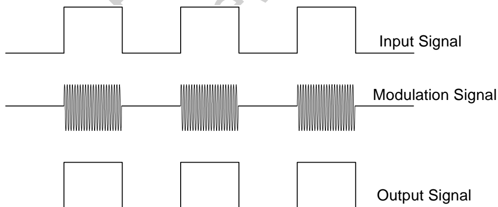
Figure 4. Modulation Scheme
