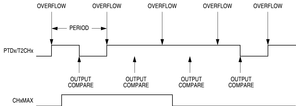
Figure 18-9. CHxMAX Latency
