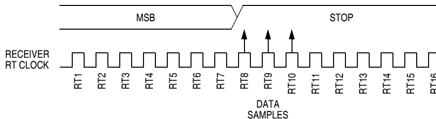
Figure 13-8. Slow Data
