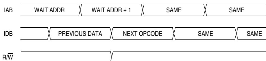
Figure 14-16. Wait Mode Entry Timing
