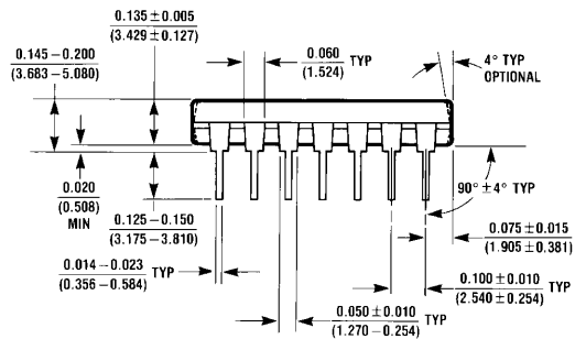
Molded Dual-In-Line Package (N) Order Number DS1489N or DS1489AN NS Package Number N14A
