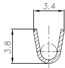
SECT "B-B"
