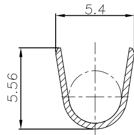
SECT "C-C"
