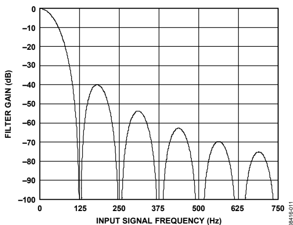
Figure 12. Filter Response
