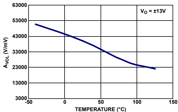
FIGURE 23. A voL vs TEMPERATURE
