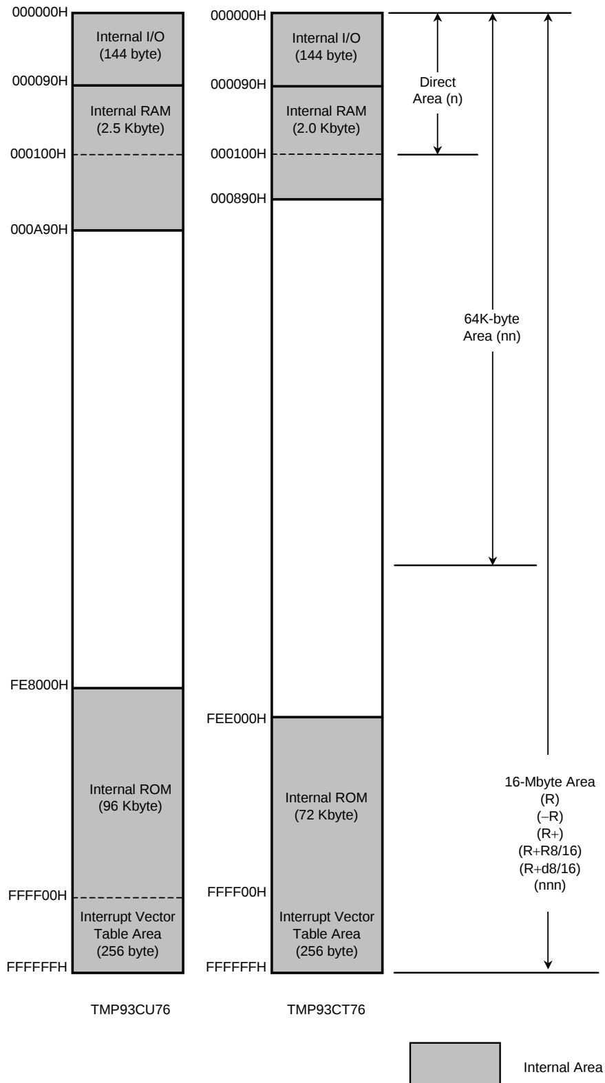
Figure 3.2.1 Memory map (2/2)
