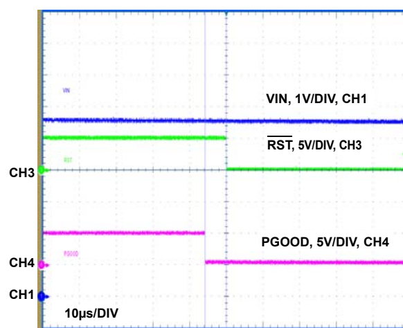
FIGURE 11. PGOOD FALLING TO \overline{RST} FALLING
