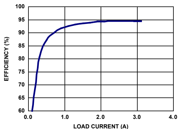
FIGURE 7. PWM3 EFFICIENCY vs LOAD ( V_O = 5V ), V_{IN} = 12V , 1 DUAL SO-8 MOSFET (IRF7907) FOR UPPER AND LOWER MOSFETS
