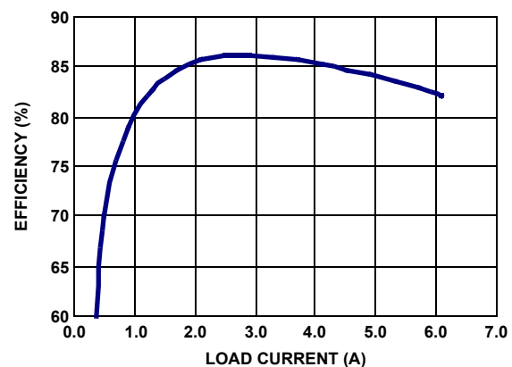
FIGURE 5. PWM2 EFFICIENCY vs LOAD ( V_O = 1.5\text{V} ), V_{\text{IN}} = 12\text{V} , 1 DUAL SO-8 MOSFET (IRF7907) FOR UPPER AND LOWER MOSFETS
