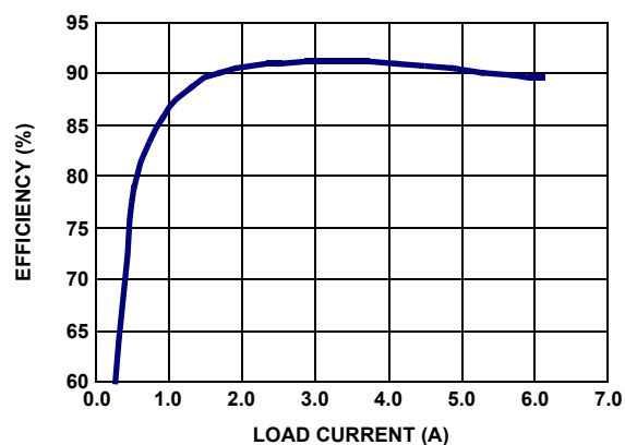
FIGURE 3. PWM1 EFFICIENCY vs LOAD ( V_O = 2.5\text{V} ), V_{\text{IN}} = 12\text{V} , 1 DUAL SO-8 MOSFET (IRF7907) FOR UPPER AND LOWER MOSFETS
