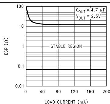
Figure 32. ESR Curves for 2.5-V Output
