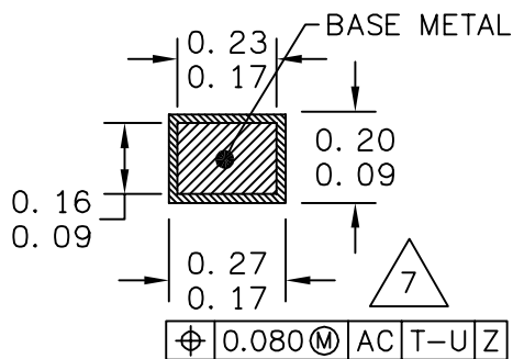
SECTION AE-AE
