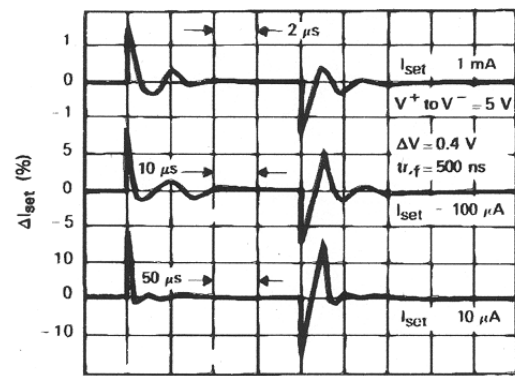
TRANSIENT RESPONSE
