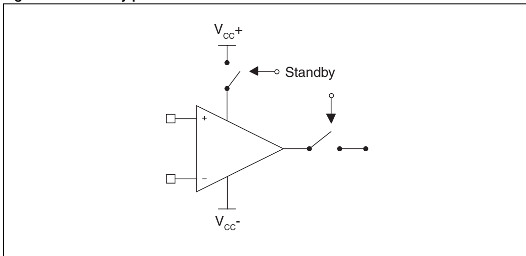
Figure 2. Standby position
