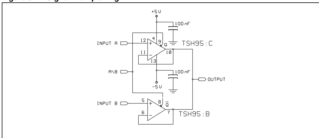
Figure 3. Signal multiplexing
