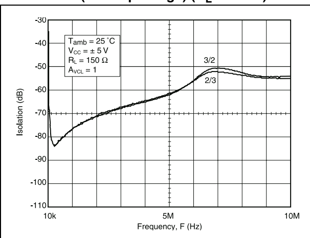
Figure 14. Crosstalk isolation vs. frequency (SO-16 package) ( R_L = 150\ \Omega )
