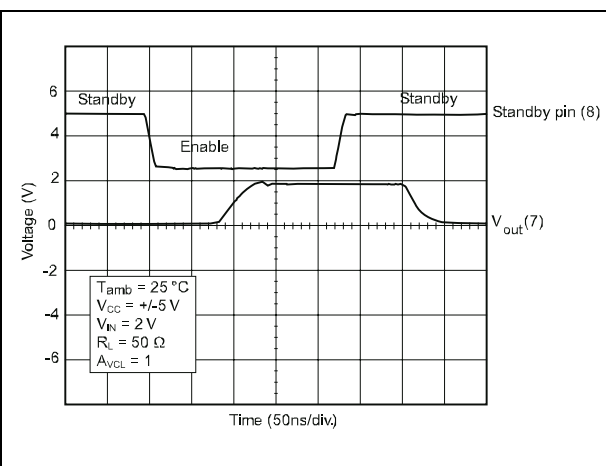
Figure 16. Standby switching
