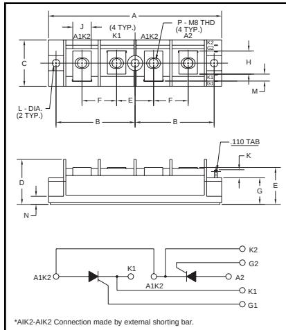
Outline Drawing
