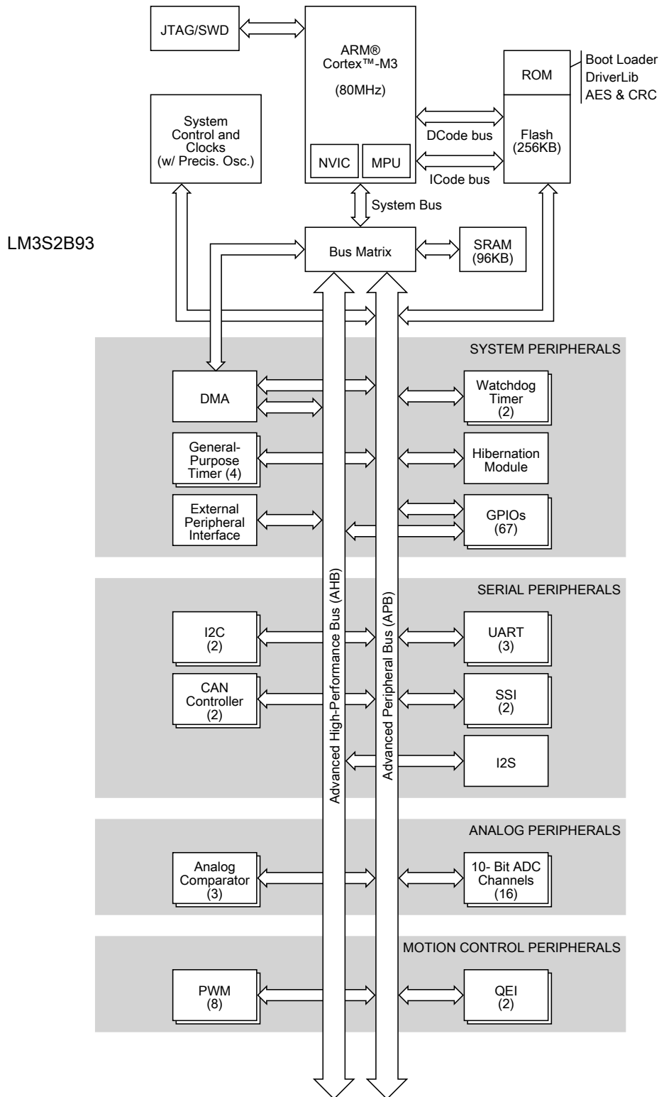
Figure 1-1. Stellaris LM3S2B93 Microcontroller High-Level Block Diagram
