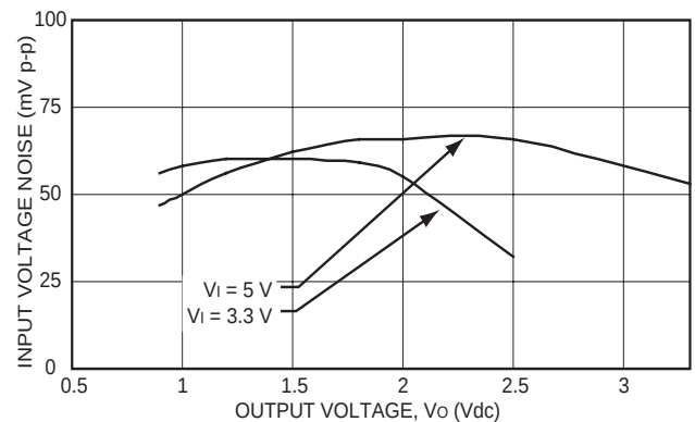
Figure 19. Input Voltage Ripple for Various Output Models, I_O = 10\text{ A} ( C_{IN} = 3 \times 150\mu F polymer // 2 \times 47\mu F ceramic).
