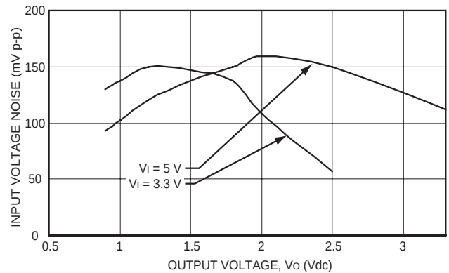
Figure 18. Input Voltage Ripple for Various Output Models, I_O = 10\text{ A} ( C_{IN} = 150\mu F polymer // 47\mu F ceramic).
