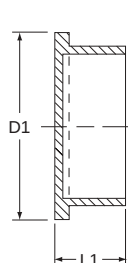
For Plugs
