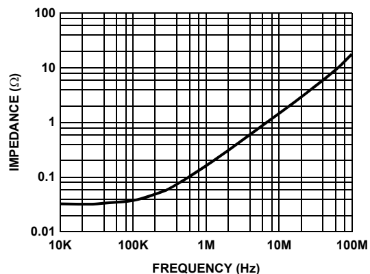
FIGURE 13. OUTPUT IMPEDANCE vs FREQUENCY
