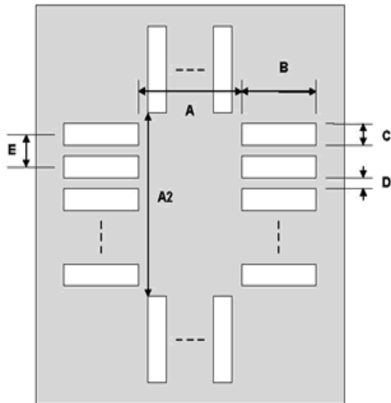
Top View (SMT Footprint)
