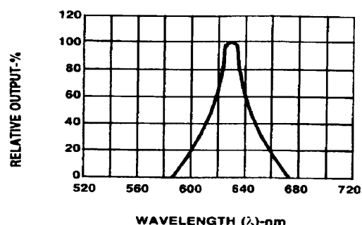
Fig.2 SPECTRAL RESPONSE
