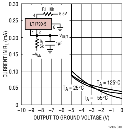
-5V Characteristics
