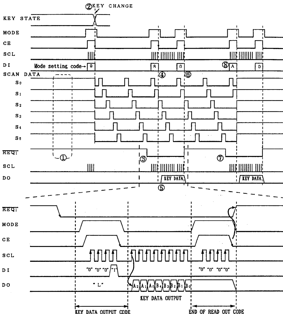
(3-3) Key Scan Timing Chart
