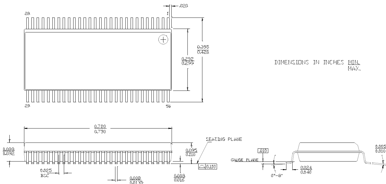
56-Lead Shrink Small Outline Package O56
