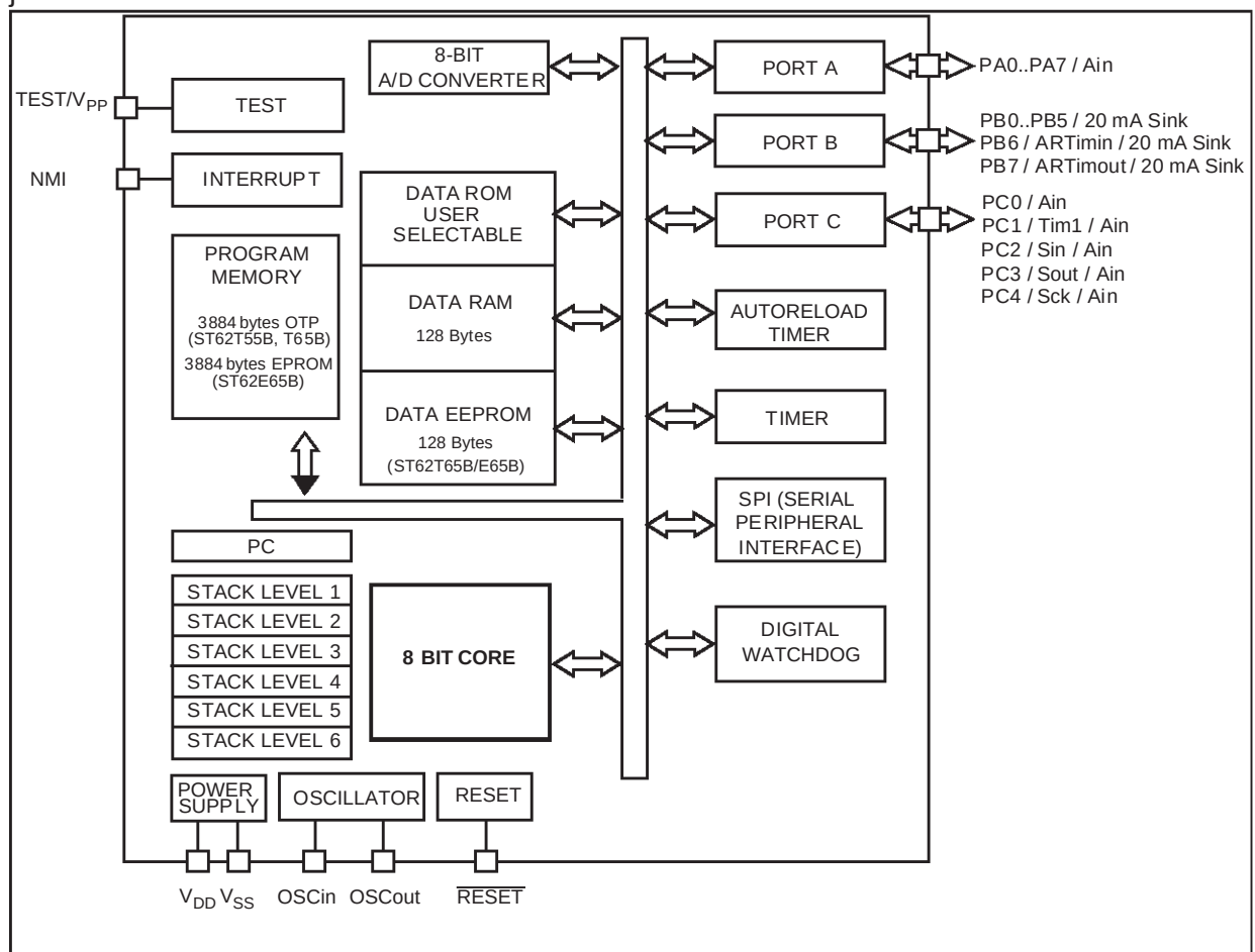
Figure 1. Block Diagram
