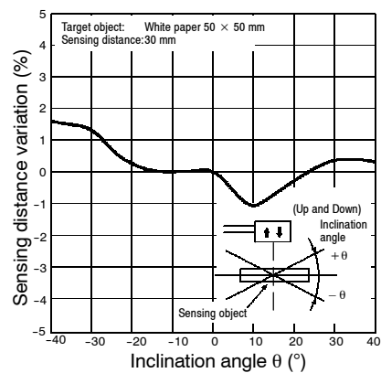
E3G-L1□ (Up and Down)
