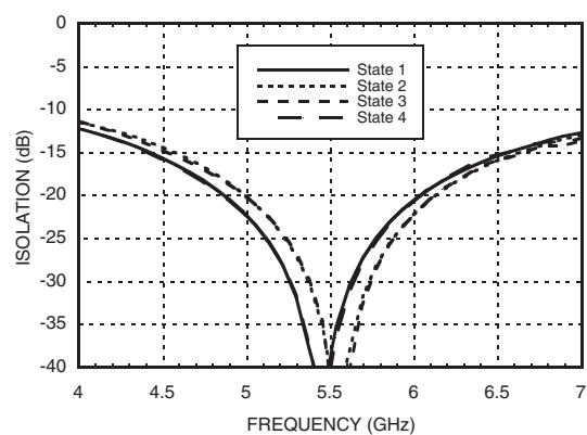
Isolation, ANT1 & ANT2
