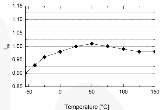
Figure 11. Feedback Source Current ( I_{FB} ) vs. T_A
