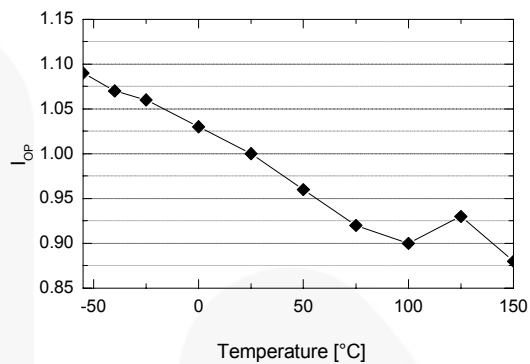
Figure 5. Operating Supply Current ( I_{\text{OP}} ) vs. T_A
