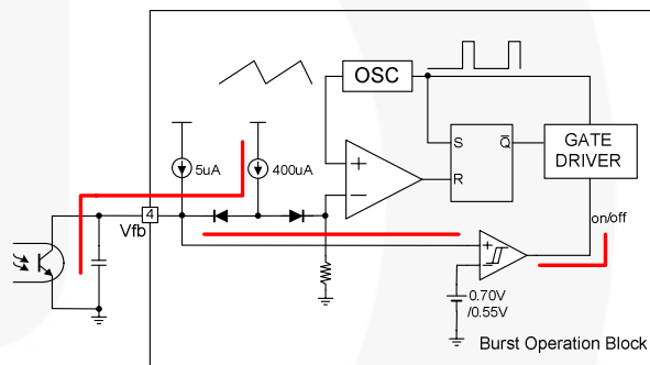
Figure 21. Burst Operation Block
