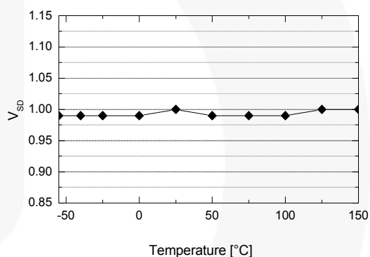
Figure 13. Shutdown Feedback Voltage ( V_{SD} ) vs. T_A
