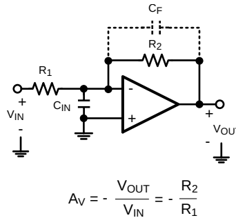
Figure 46. Inverting Amplifier
