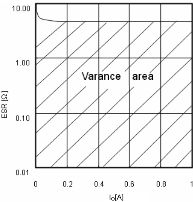
Fig.18 ESR condencer
