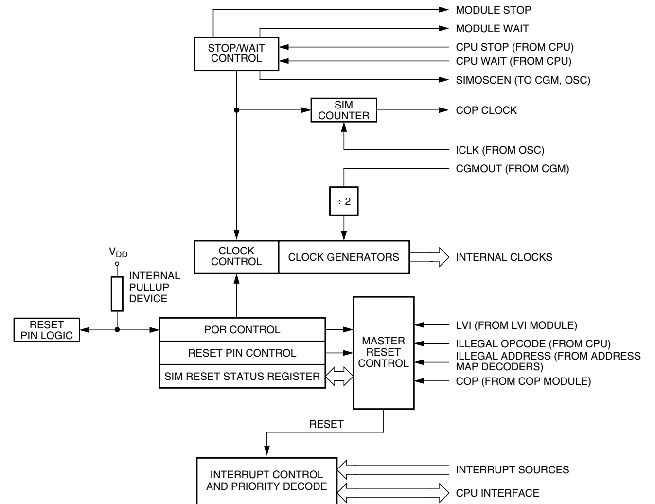
Figure 7-1. SIM Block Diagram
