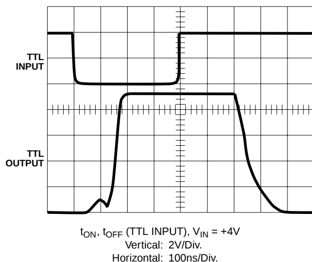
FIGURE 7. TTL INPUT
