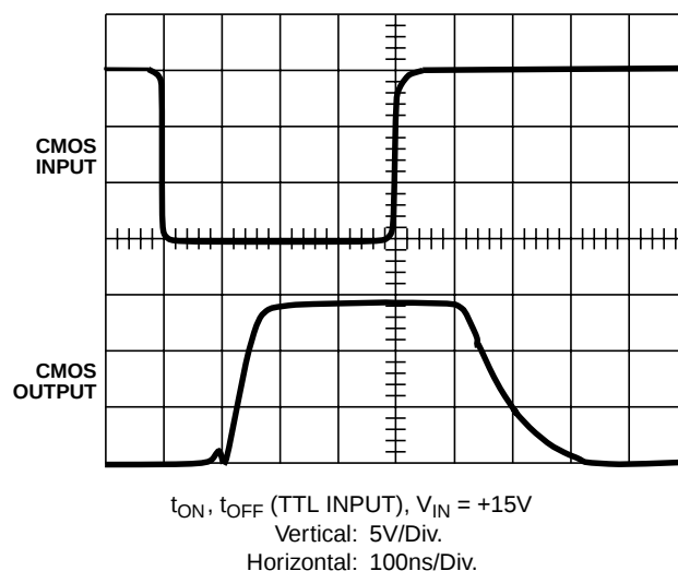
FIGURE 7. TTL INPUT
