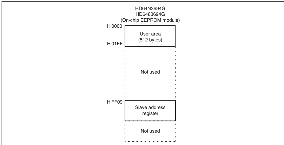
Figure 2.1 Memory Map (3)
