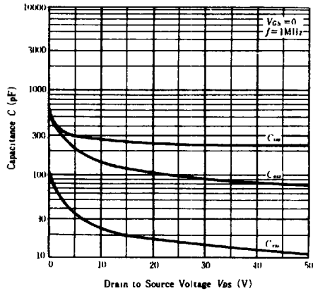
TYPICAL CAPACITANCE VS. DRAIN-SOURCE VOLTAGE
