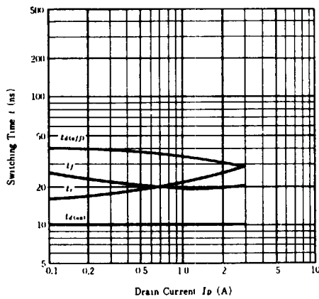
SWITCHING CHARACTERISTICS
