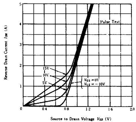
MAXIMUM BODY-DRAIN DIODE
