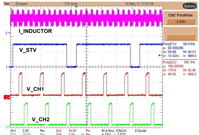
FIGURE 17. V_{\text{SYNC}} ENABLED WITH PHASE SHIFT ( V_{\text{IN}} : 19V, I_{\text{CH}} : 120mA, LEDs: 4P18S, 180Hz OUTPUT PHASE AND FREQUENCY LOCKED TO 60Hz STV)
