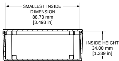
SECTION L-L
