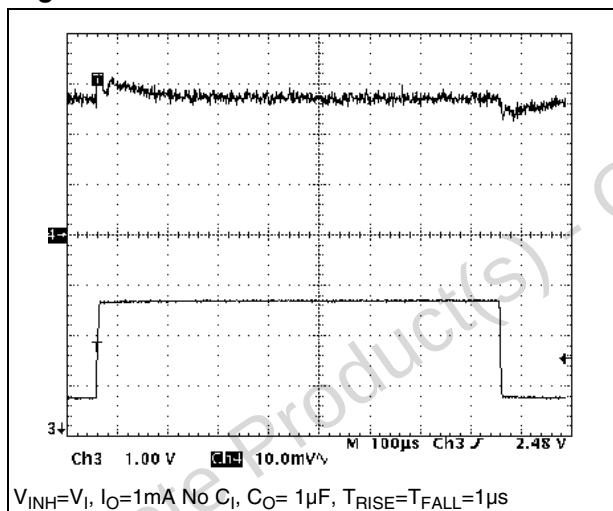
Figure 11. Line transient
