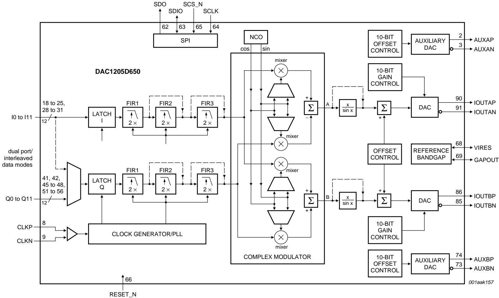
Fig 1. Block diagram
