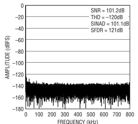
32k Point FFT f_{\text{S}} = 1.6\text{Msps} , f_{\text{IN}} = 2\text{kHz}
