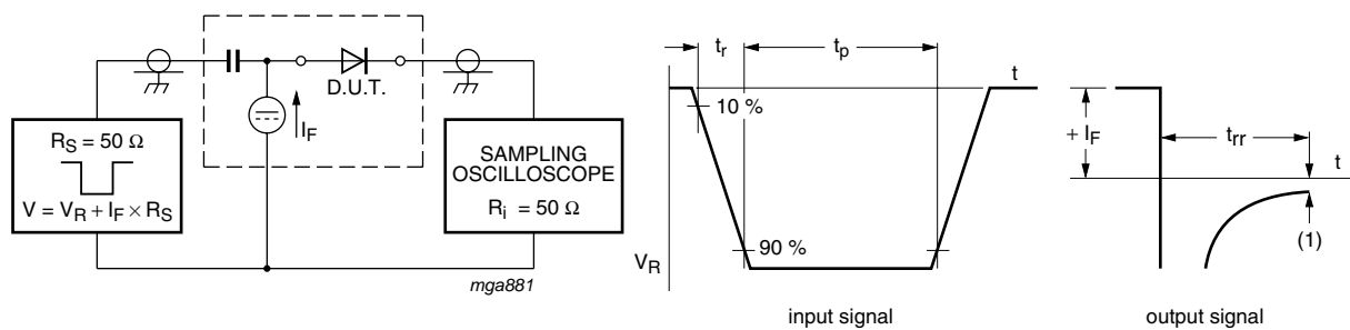
(1) I_R = 3\text{ mA} Fig 6. Reverse recovery time test circuit and waveforms
