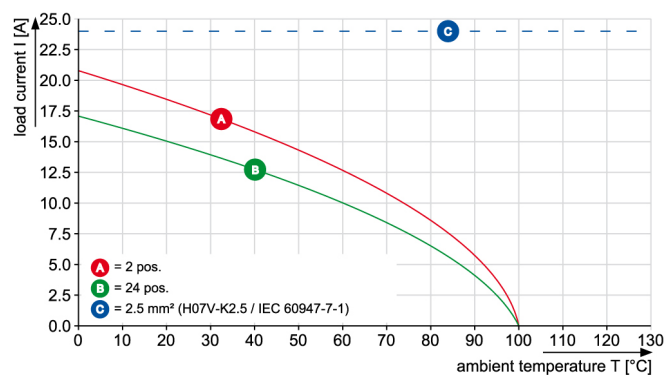
BLT 5.08/..180 - SL 5.08/..90
