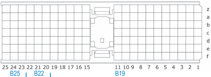
Type-A Connector
