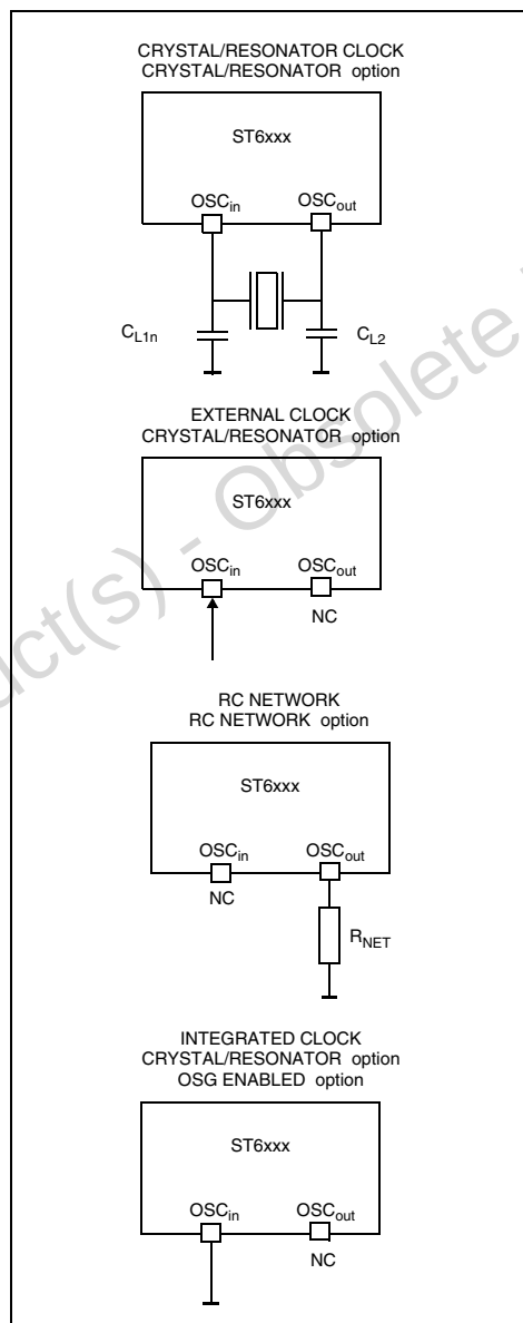
Figure 8. Oscillator Configurations
