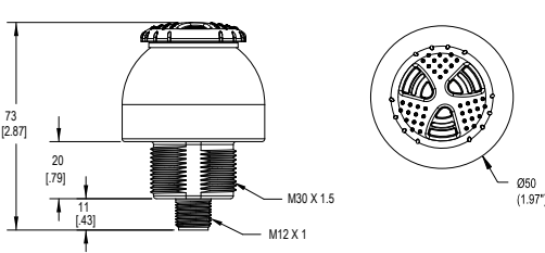
Quick-Disconnect Dimensions
