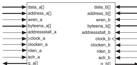
Figure 3-11. Cyclone III Device Family True Dual-Port Memory (1)
