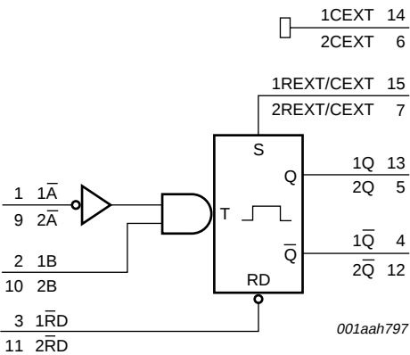
Fig 2. Logic symbol
