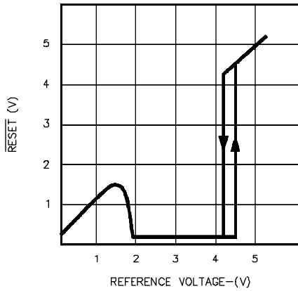
FIGURE 8. UNDERTENSION LOCKOUT CHARACTERISTIC
