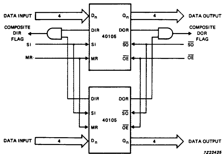
Fig.17 Expanded FIFO for increased word length; 16 words × 8 bits.
