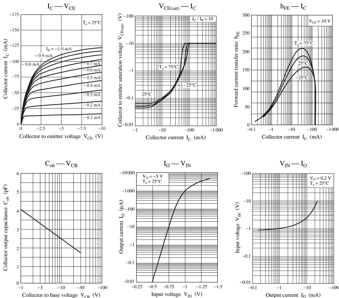
Characteristics chart of UNR911TJ
