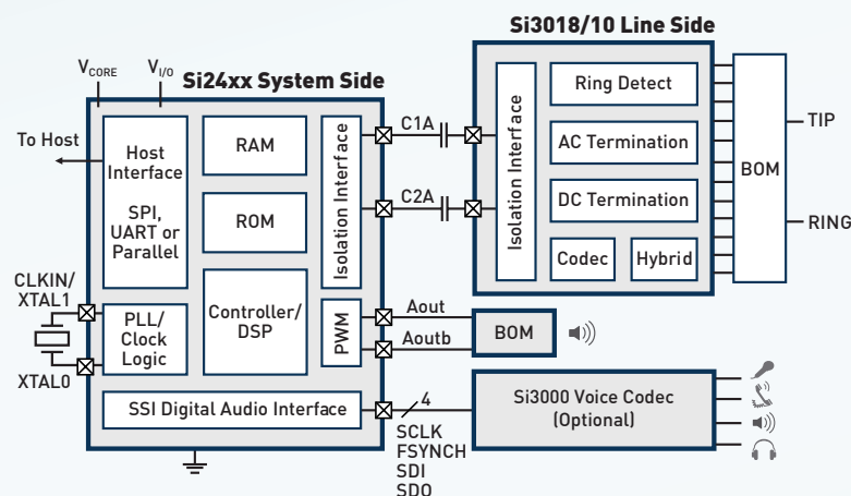
ISOmodem BLOCK DIAGRAM
