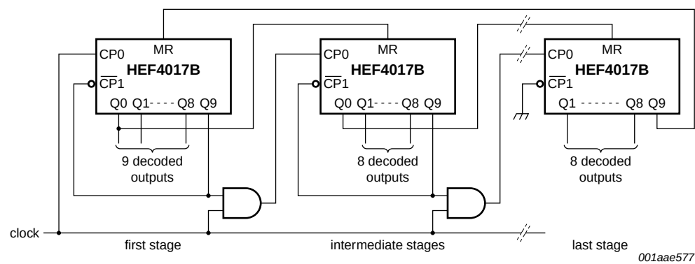
Fig 11. Counter expansion
