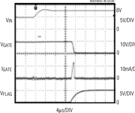
OVERVOLTAGE RESPONSE
